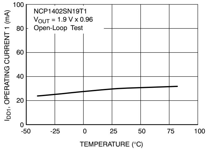
Figure 12. NCP1402SN19T1 Operating Current 1 vs. Temperature
